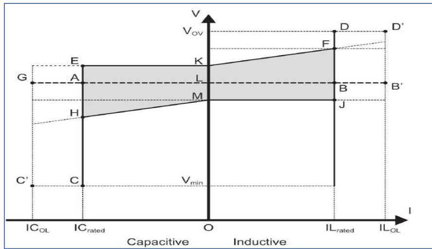
Figure-2: VI Curve of the VSC Portion
