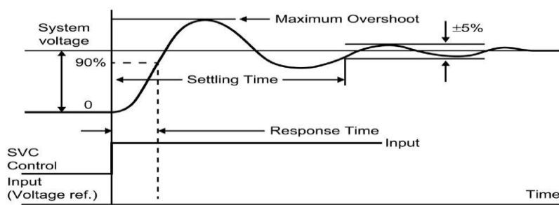
Figure-4: Response and Settling time
